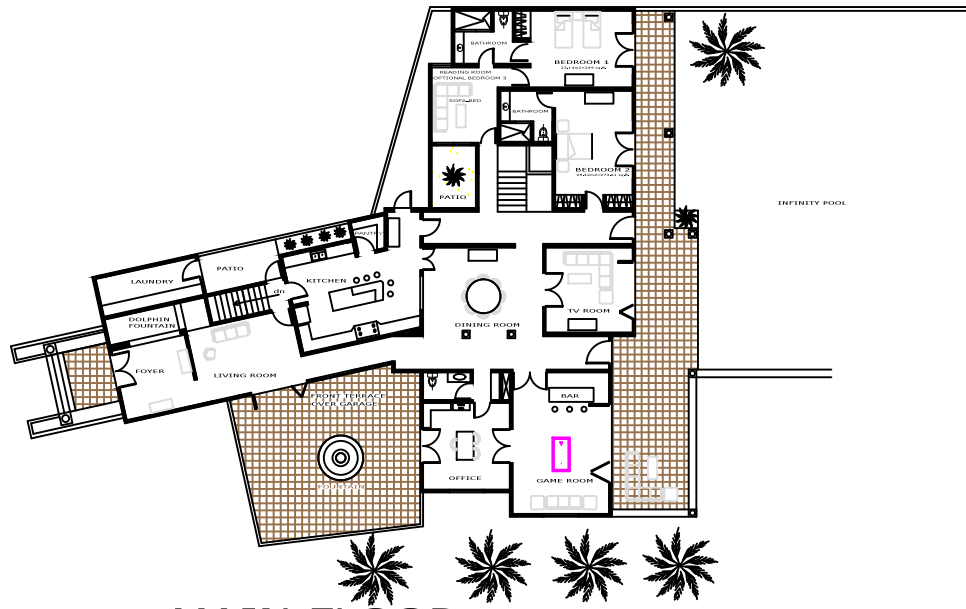
MAIN FLOOR 602m2=6,477 sq.ft.
