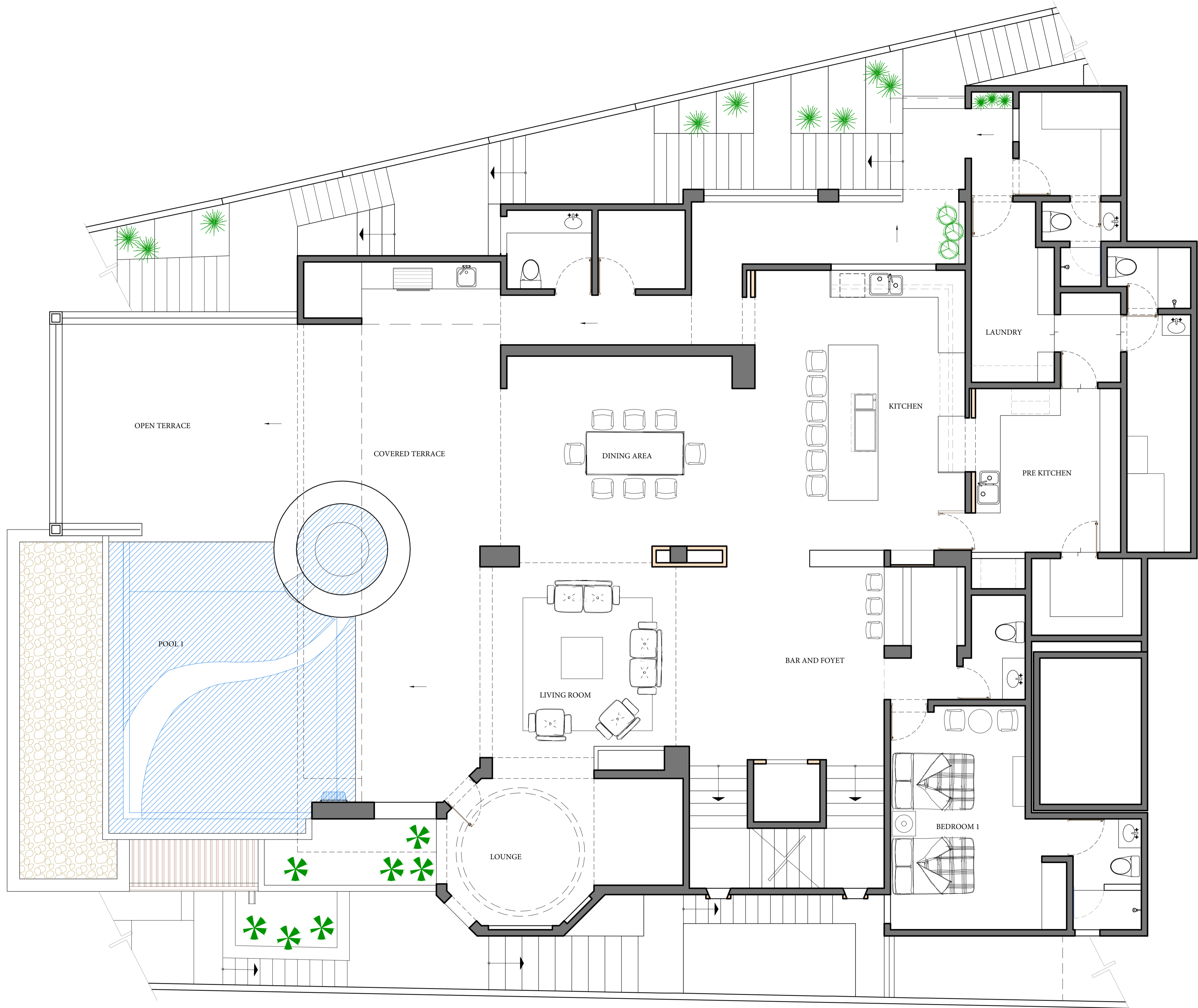
SECOND LEVEL
